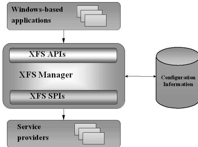
Figure 2.1 - Extensions for Financial Services Architecture
